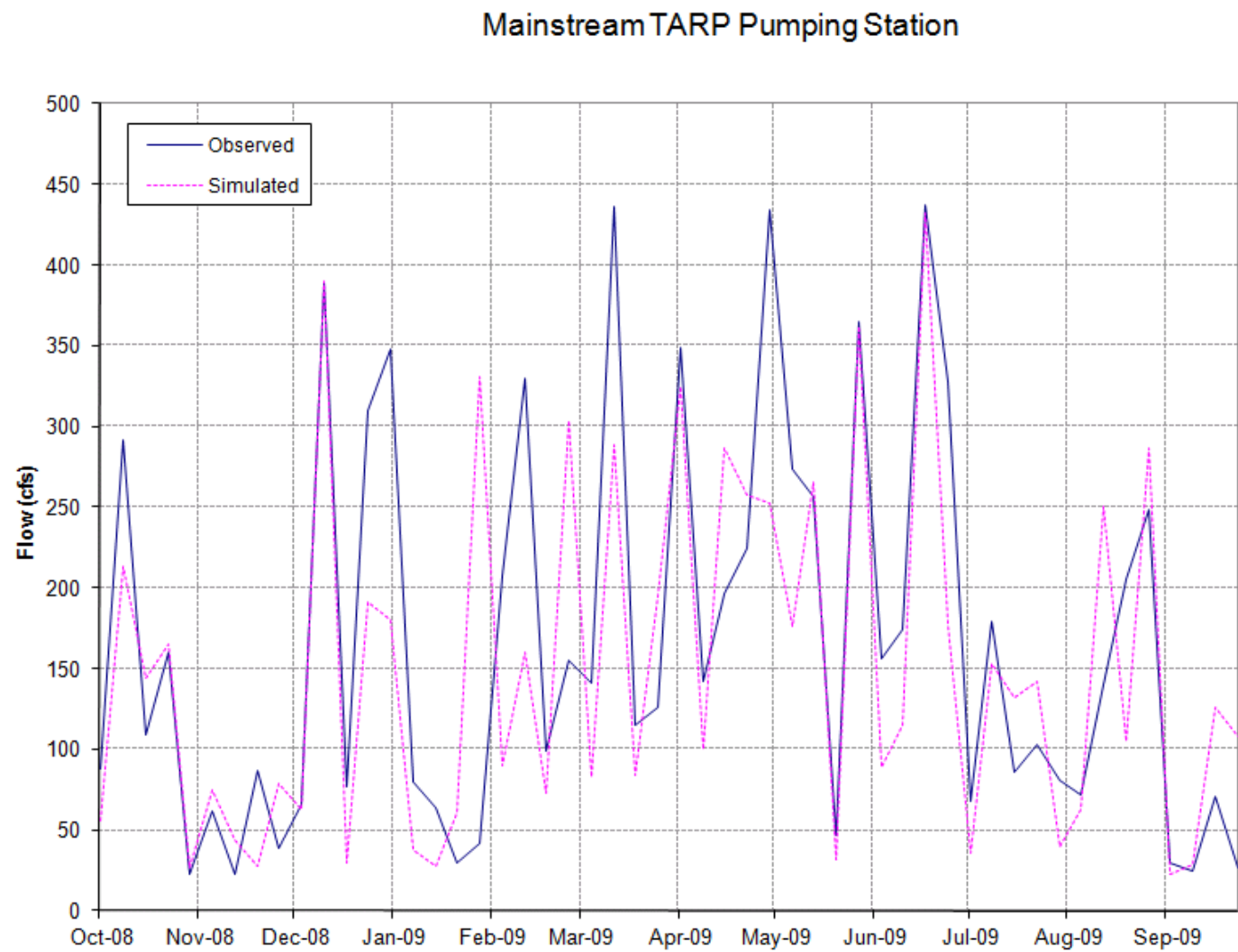
Figure 7 Budget 9 - Simulation of the MWRDGC Mainstream and Des Plaines TARP Pumping Station
