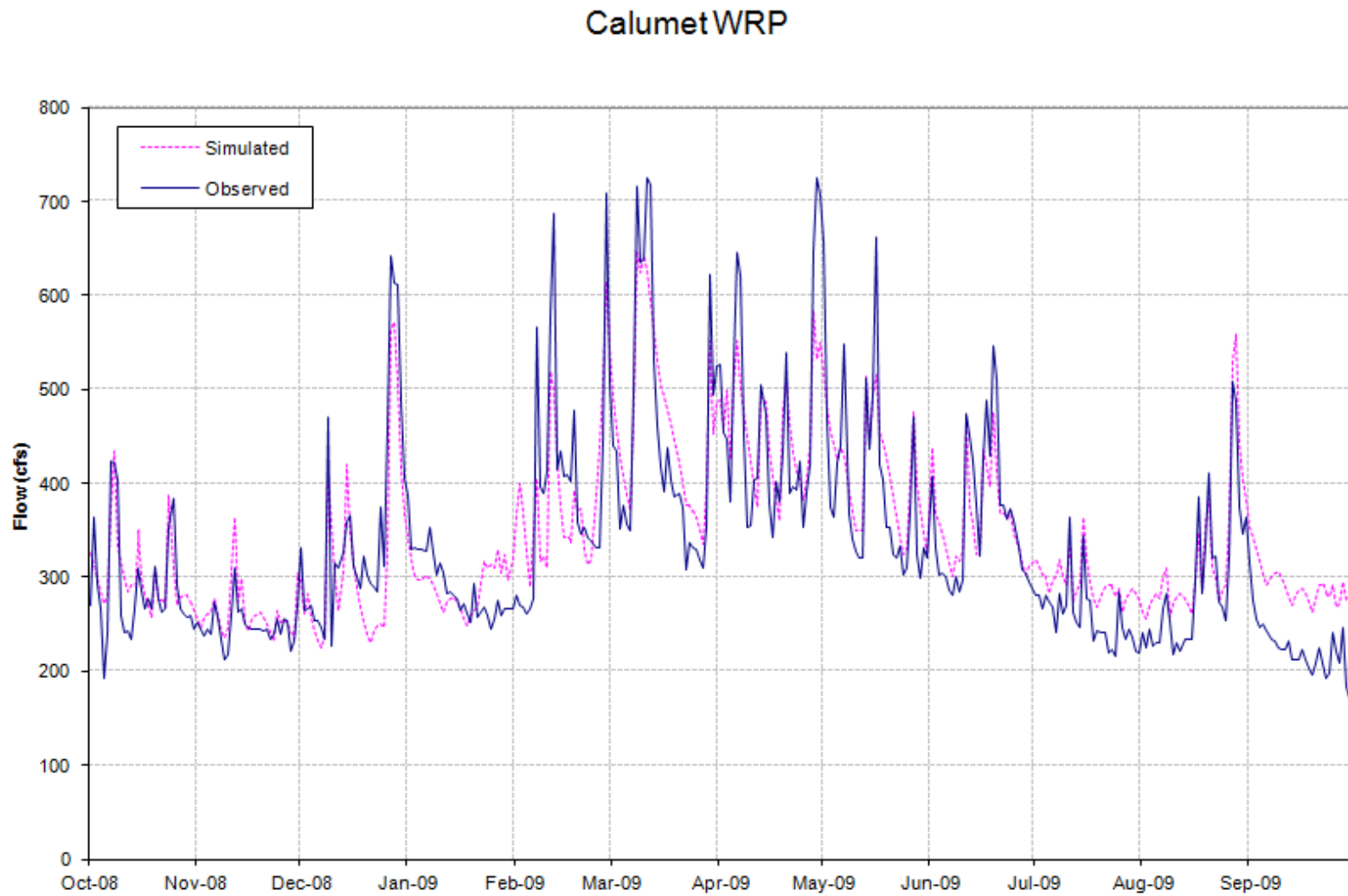
Figure 10 Budget 12 – Simulation of the MWRDGC Calumet Water Reclamation Facility
