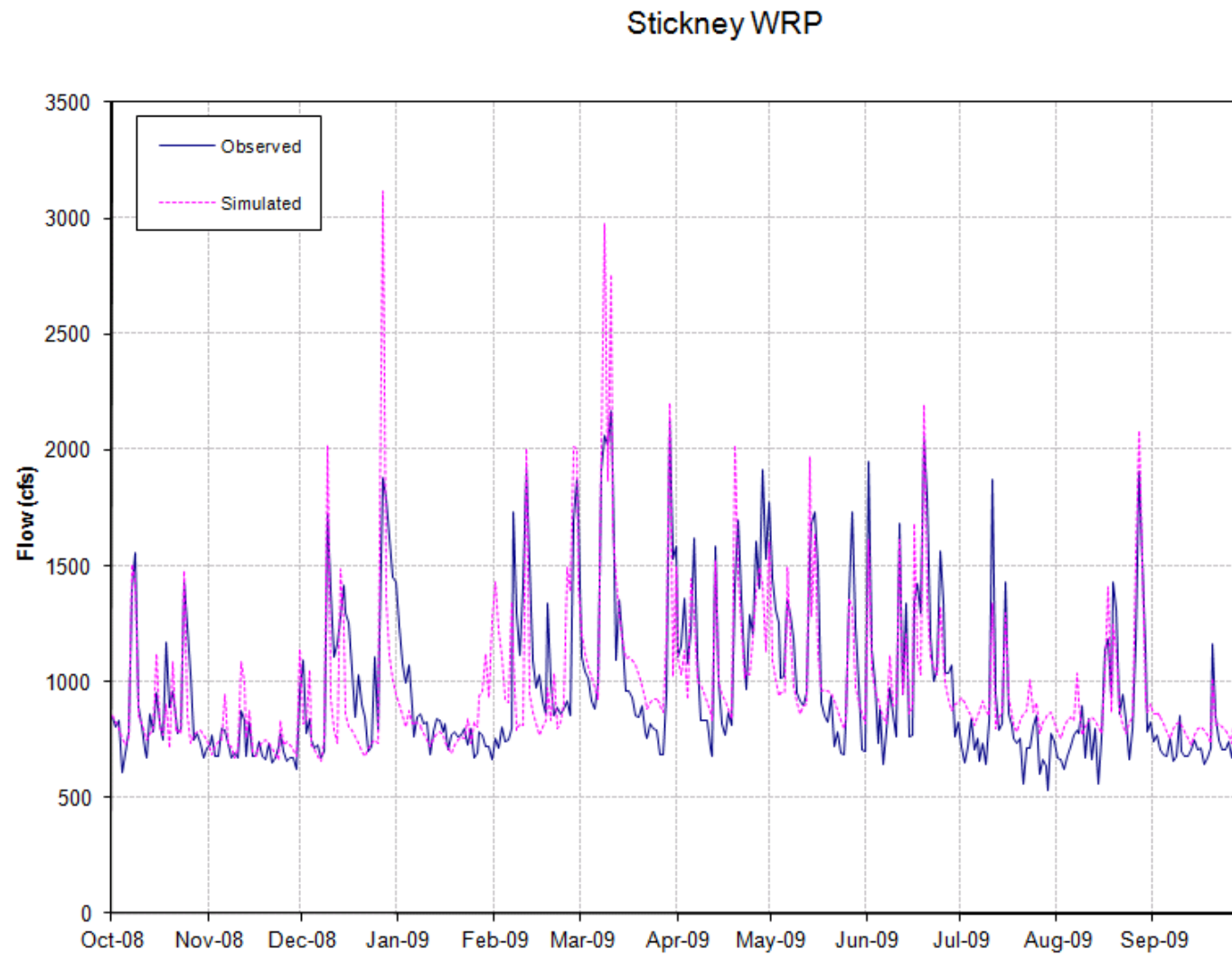
Figure 8 Budget 10 - Simulation of the MWRDGC Stickney Water Reclamation Facility
