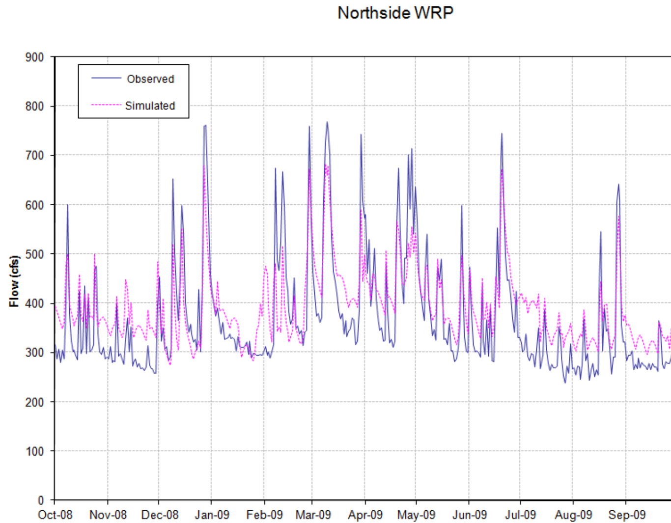
Figure 4 Budget 7 - Simulation of the MWRDGC Northside Water Reclamation Facility
