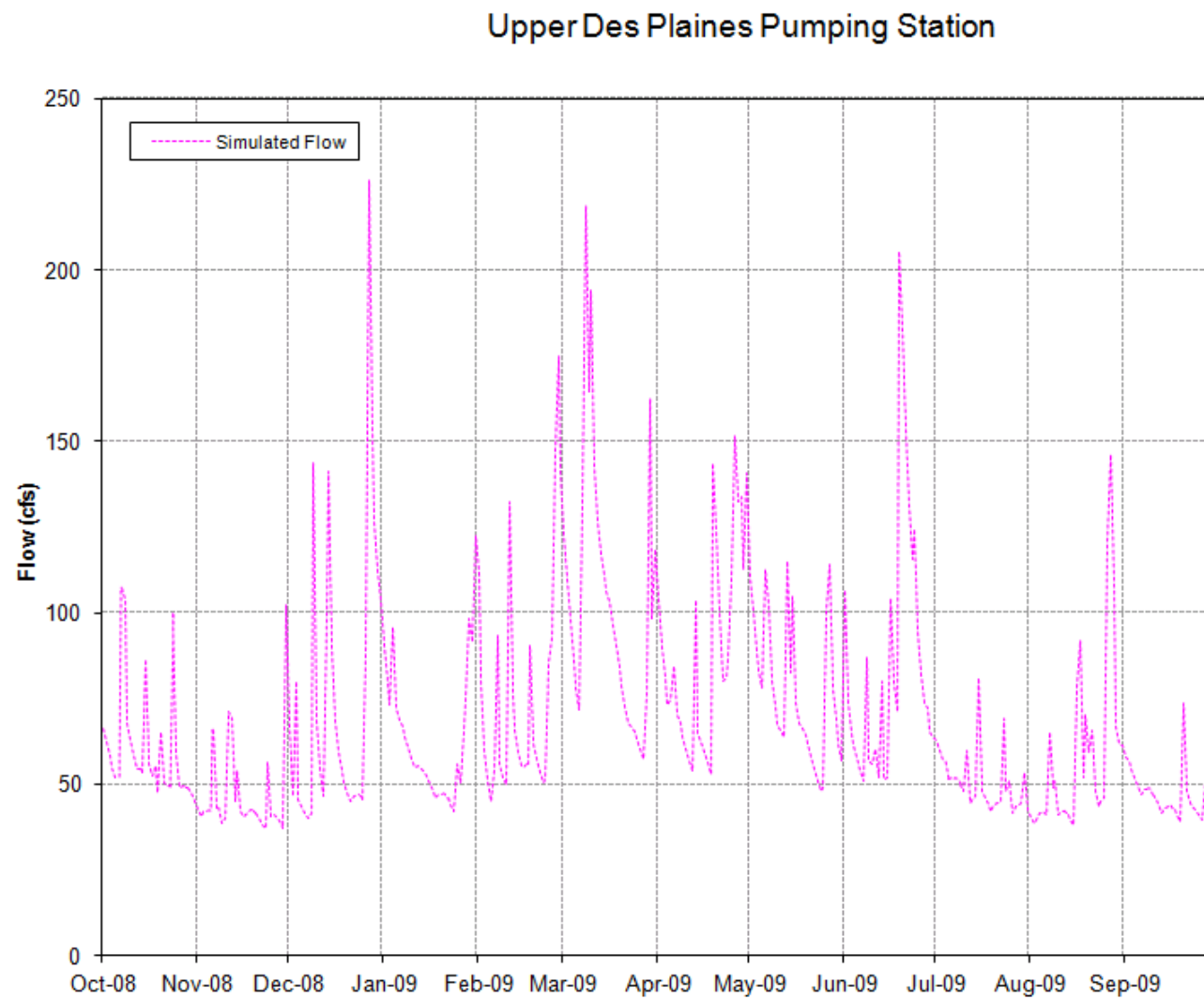
Figure 5 Budget 8 - Simulation of the MWRDGC Upper Des Plaines Pump Station
