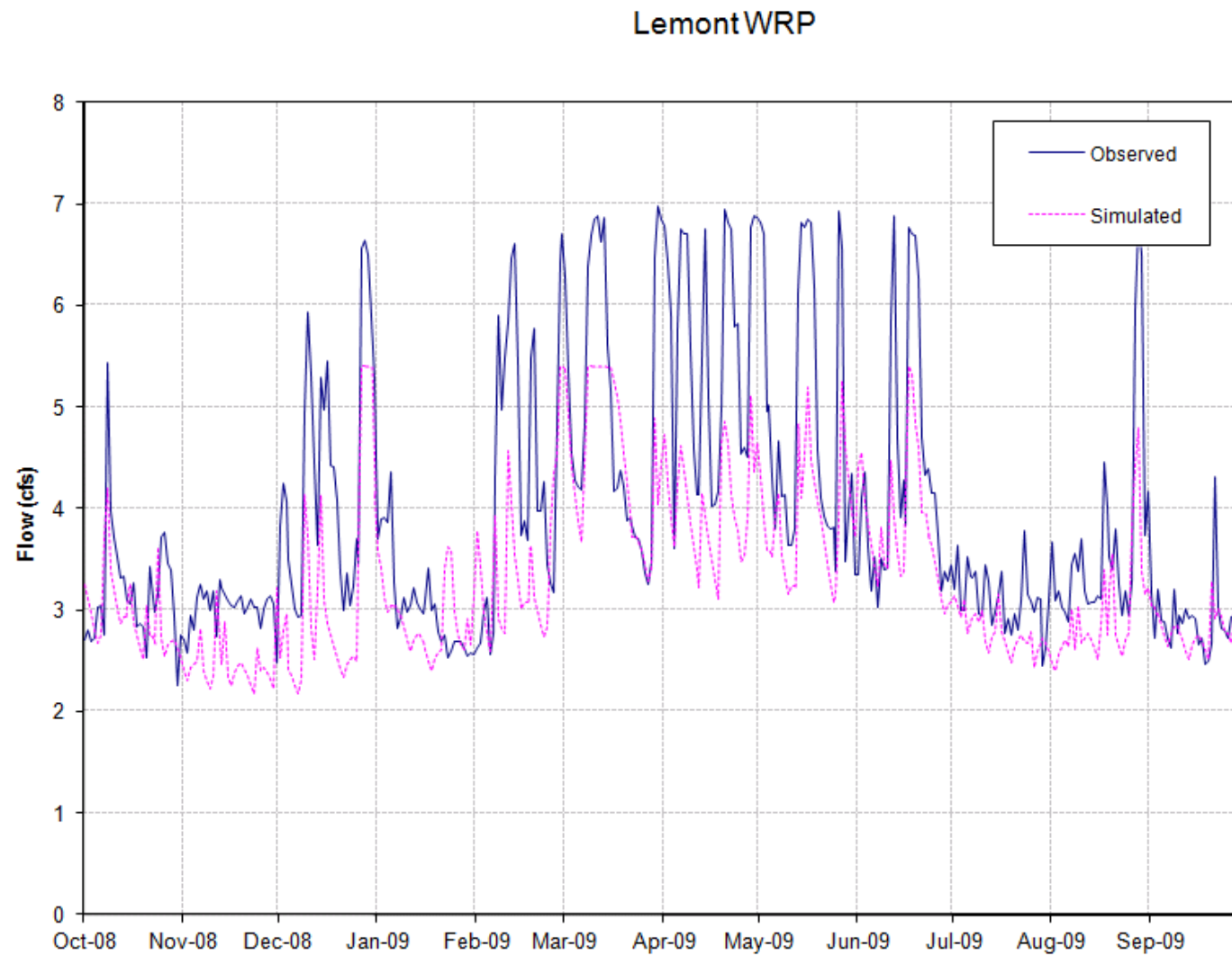
Figure 11 Budget 13 – Simulation of the MWRDGC Lemont Water Reclamation Facility
