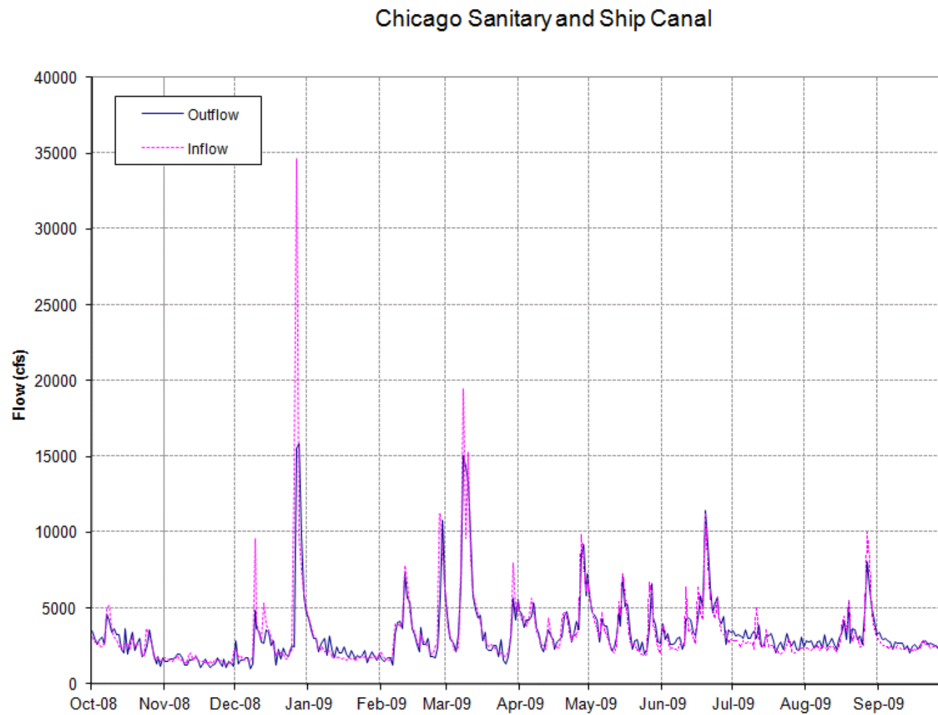
Figure 12 Budget 14 – CSSC System Balance
