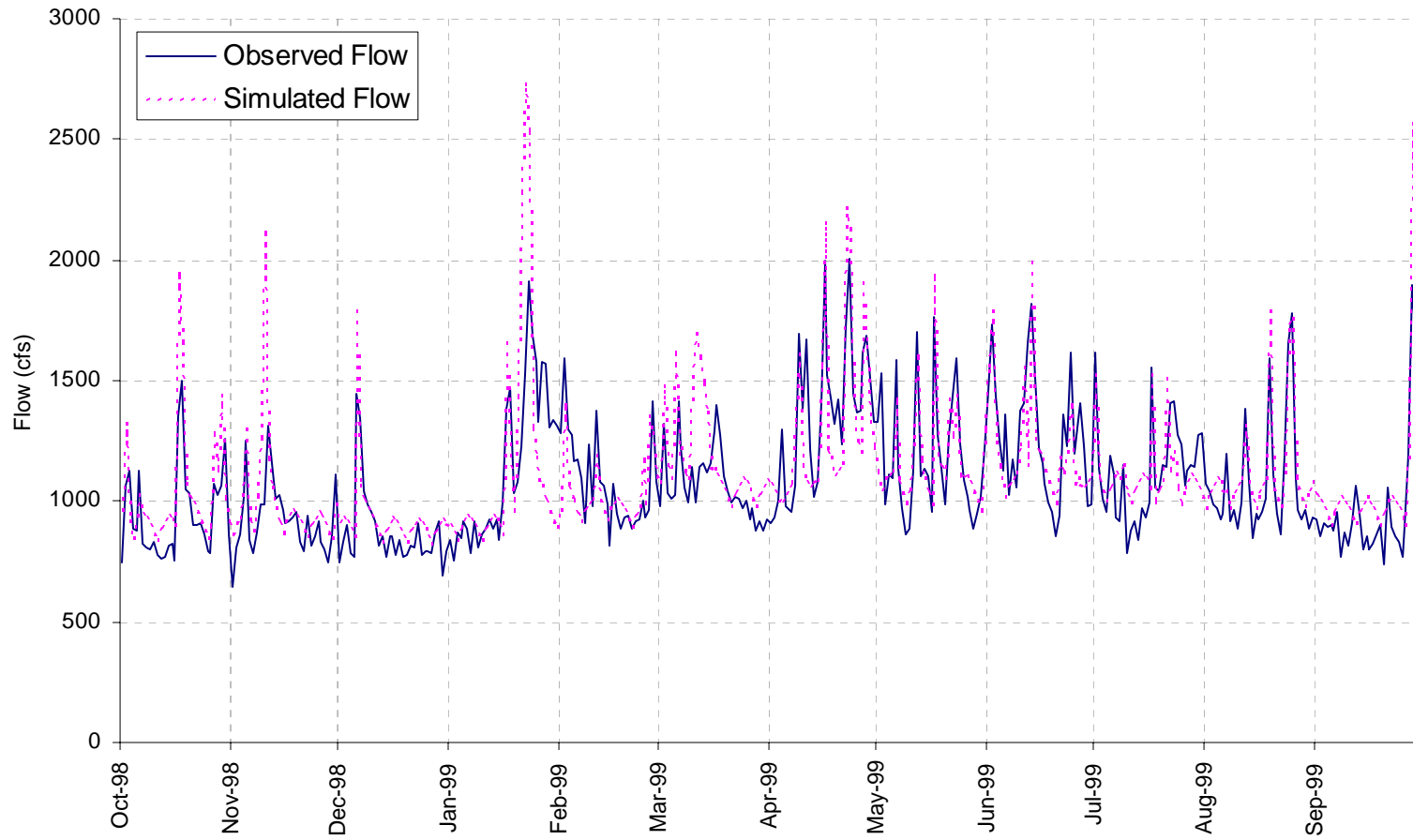
Figure 8 Budget 10 - Simulation of the MWRDGC Stickney Water Reclamation Facility
