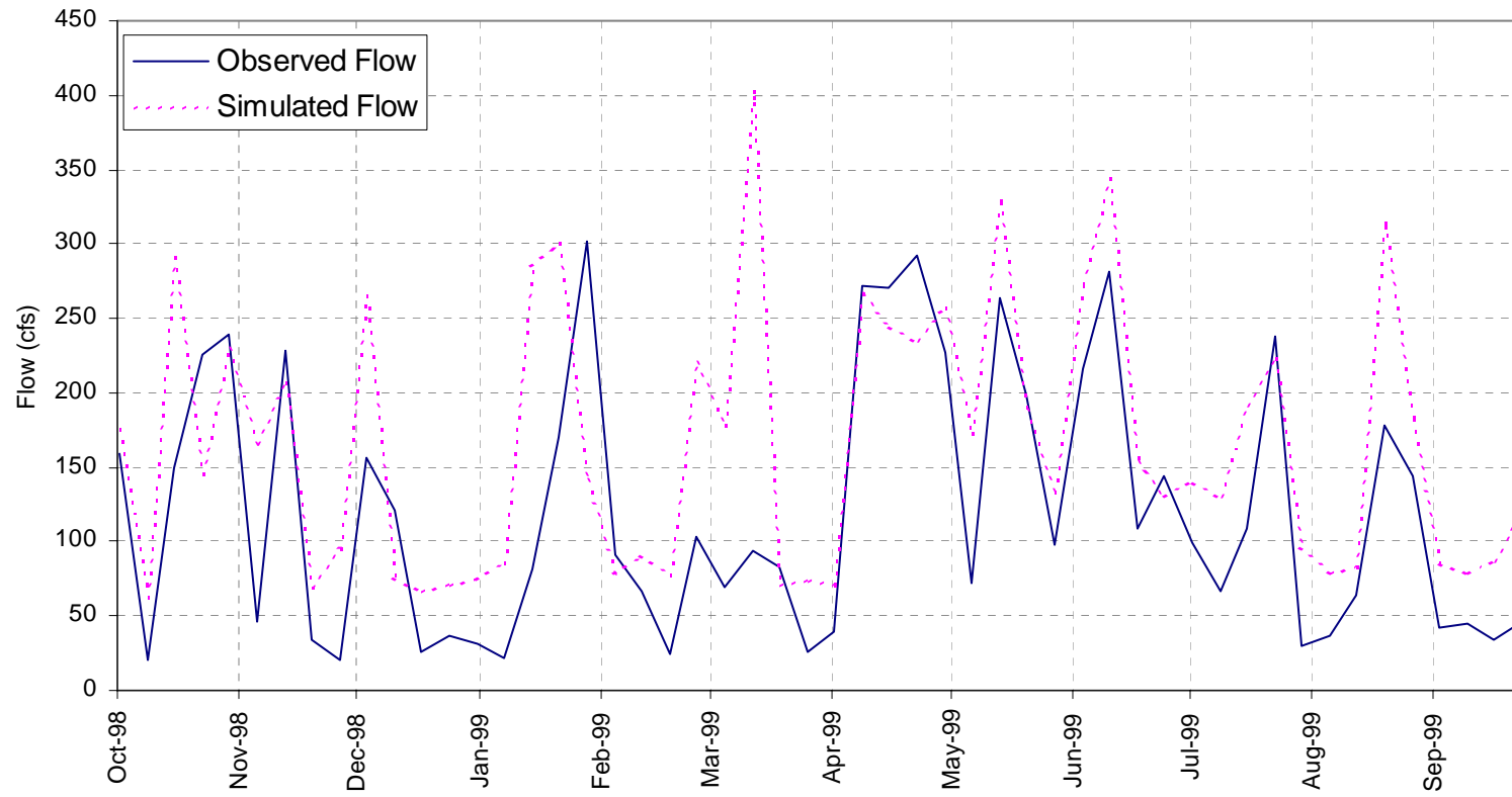
Figure 7 Budget 9 - Simulation of the MWRDGC Mainstream and Des Plaines TARP Pumping Station
