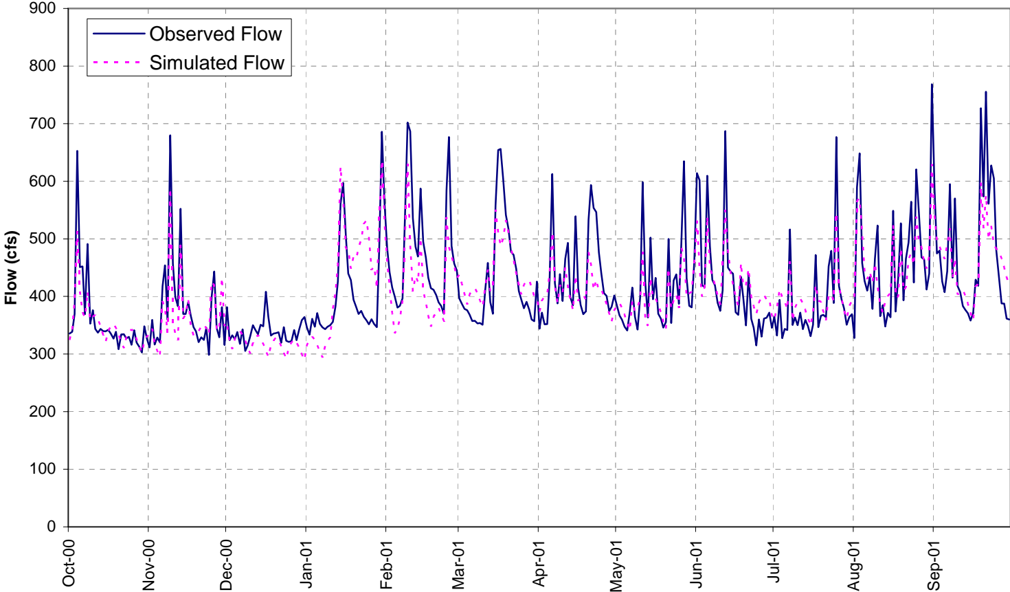
Figure 4 Budget 7 - Simulation of the MWRDGC Northside Water Reclamation Facility
