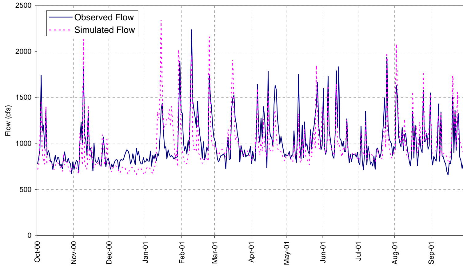
Figure 8 Budget 10 - Simulation of the MWRDGC Stickney Water Reclamation Facility
