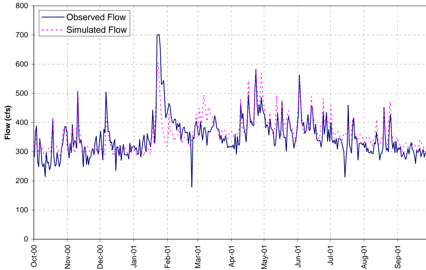
Figure 10 Budget 12 – Simulation of the MWRDGC Calumet Water Reclamation Facility
